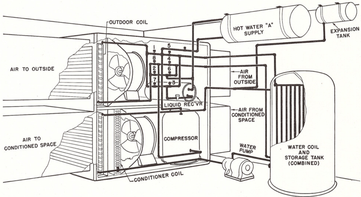
FIG. 2-9. Air-to-Water System Using Storage Tank (See Fig. 2-5)
